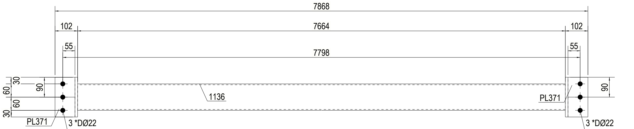
FRONT VIEW
